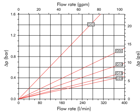
By-pass F280-D120/24/21
