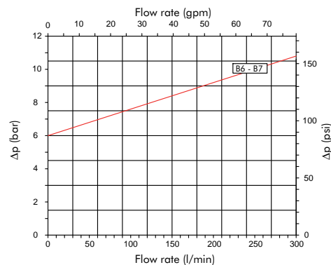
By-pass F280-D140/41/43
